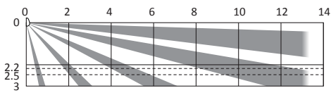
Air2-QIR200W – Side view
