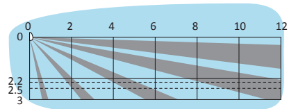
Air2-QDT200W – Side view
