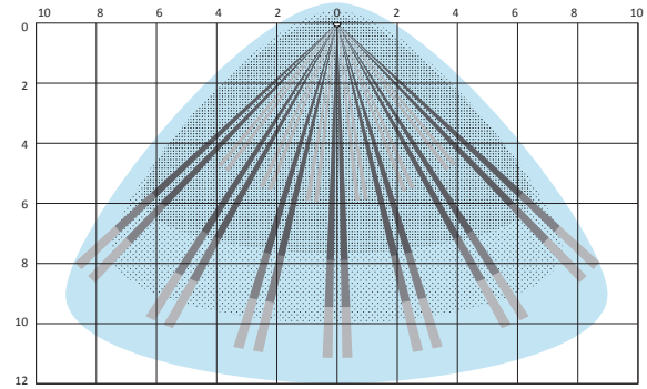
Air2-QDT200W – Top view
